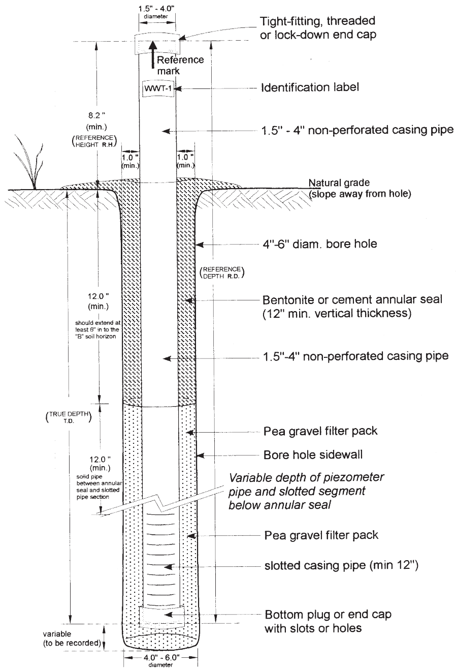
Figure 1. CROSS SECTION OF TYPICAL GROUNDWATER PIEZOMETER
