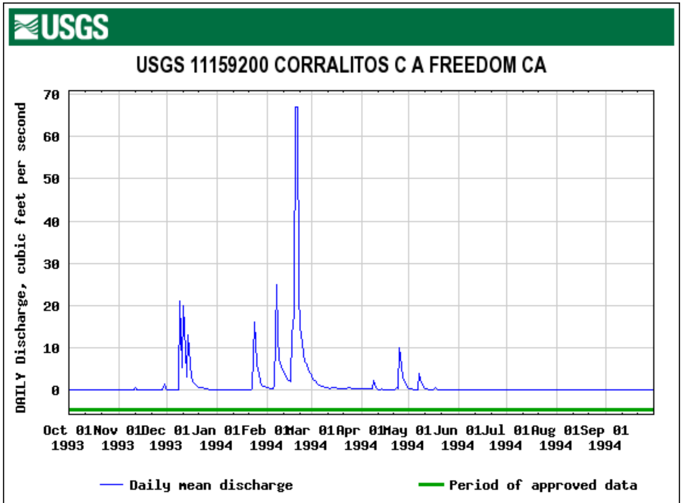
Figure 43. The 1994 Daily Mean Flow at the USGS Gage on Corralitos Creek at Freedom. (USGS website would not provide logarithmic scale of discharge.)
