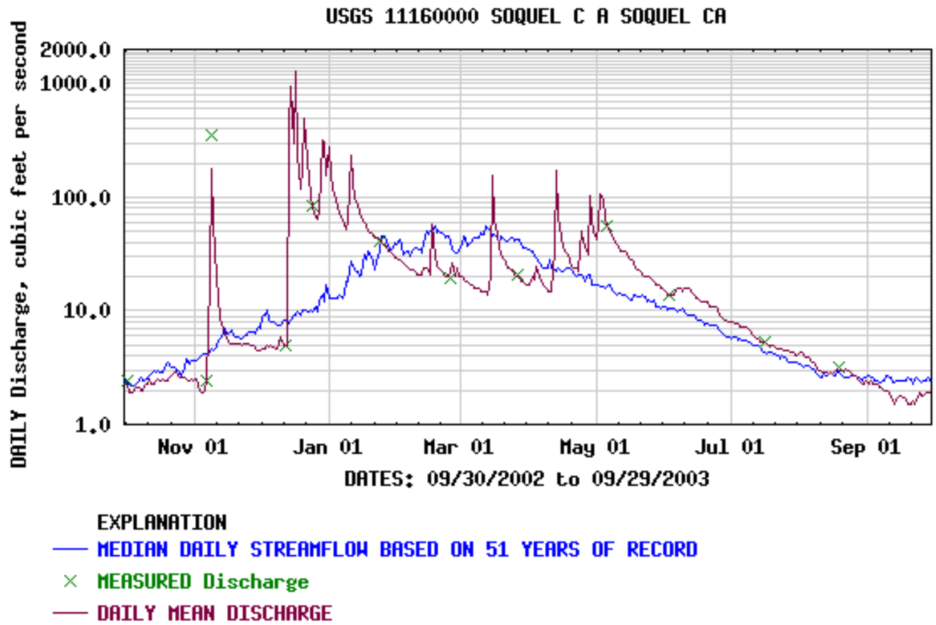
Figure 30. The 2003 Daily Mean and Median Flow at the USGS Gage on Soquel Creek at Soquel.
