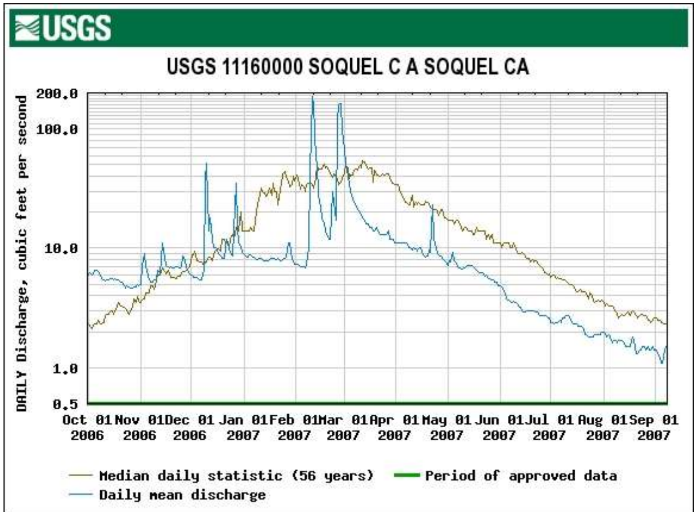
Figure 34. The 2007 Daily Mean and Median Flow at the USGS Gage on Soquel Creek at Soquel.
