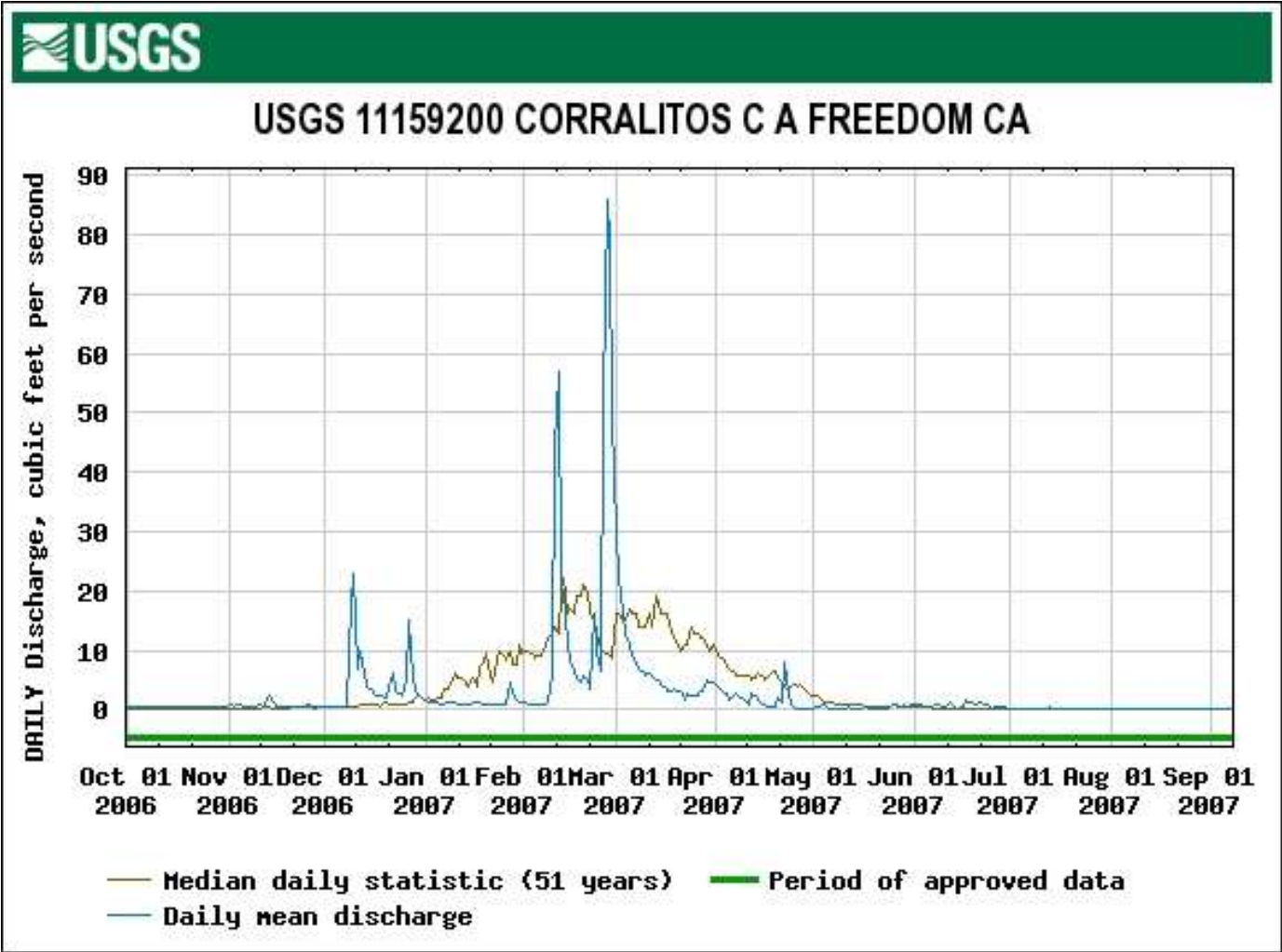
Figure 46. The 2007 Daily Mean and Median Flow at the USGS Gage on Corralitos Creek at Freedom. (USGS website would not provide a logarithmic scale of discharge).
