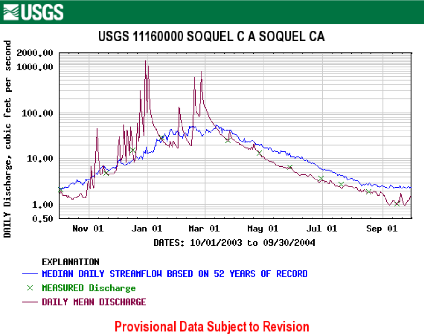
Figure 31. The 2004 Daily Mean and Median Flow at the USGS Gage on Soquel Creek at Soquel.
