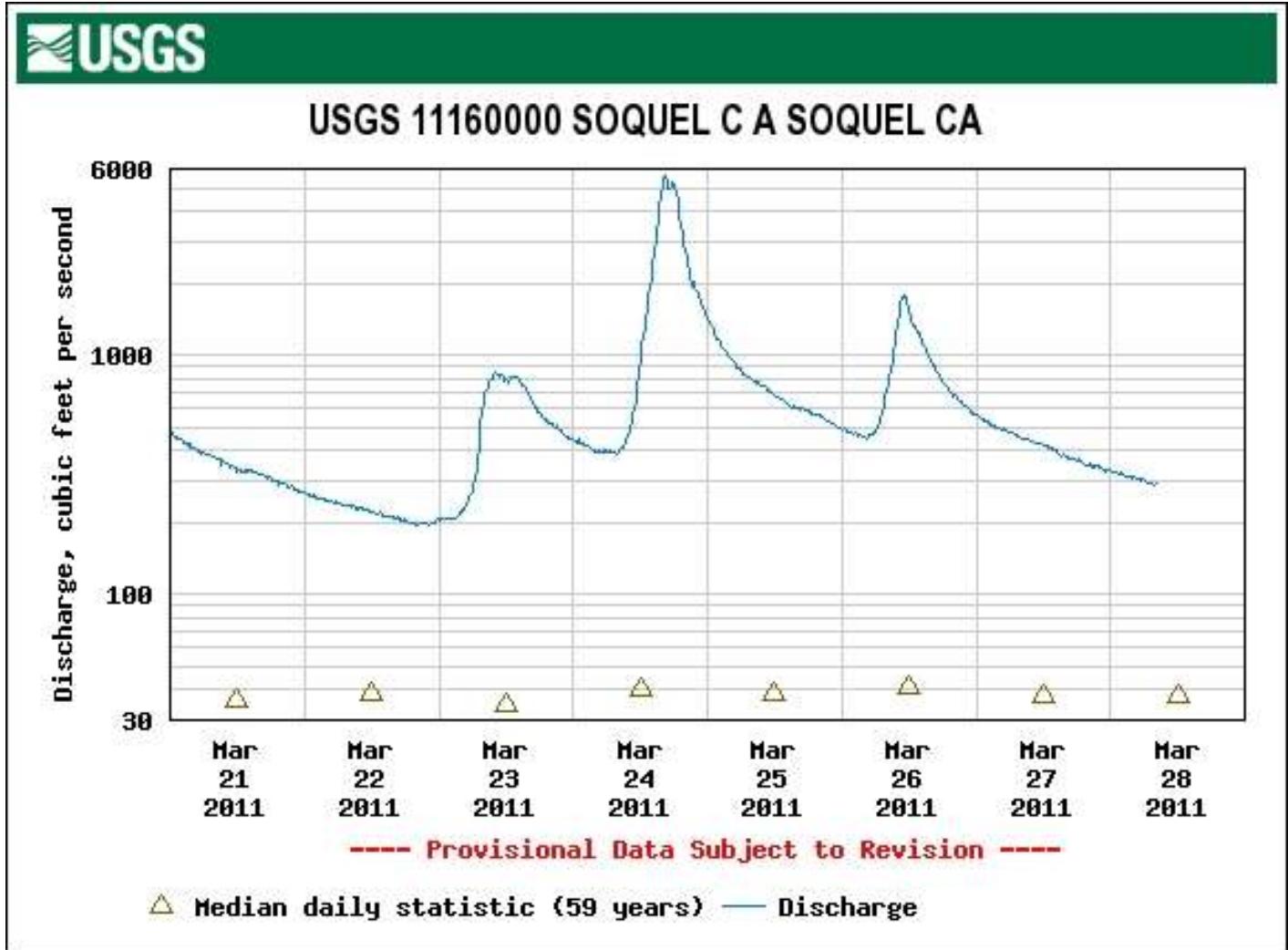
Figure 39. The Late March 2011 Discharge of Record for the USGS Gage on Soquel Creek at Soquel Village.
