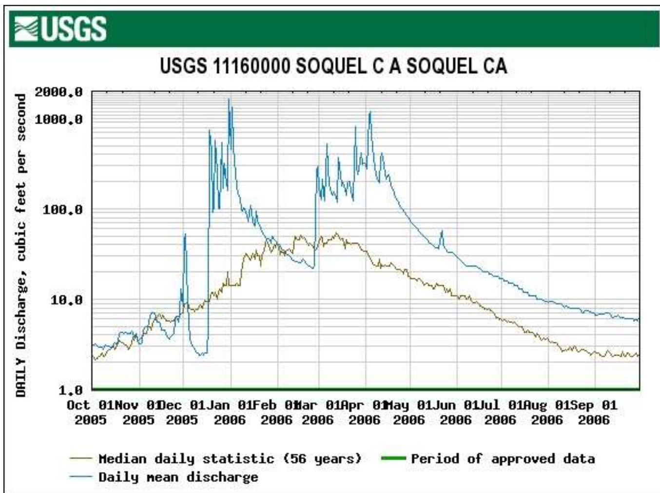
Figure 33. The 2006 Daily Mean and Median Flow at the USGS Gage on Soquel Creek at Soquel.
