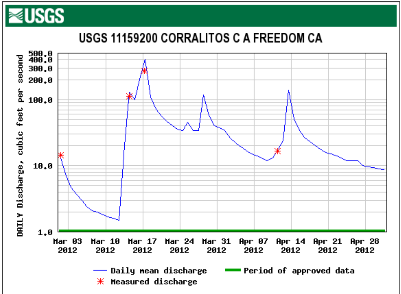
Figure 53. The March–April 2012 Discharge of Record for the USGS Gage on Corralitos Creek at Freedom.
