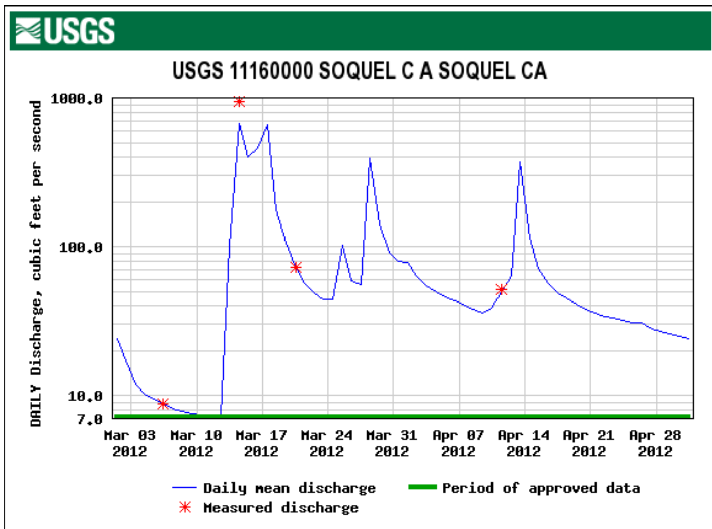
Figure 41. The March–April 2012 Discharge of Record for the USGS Gage on Soquel Creek at Soquel Village.
