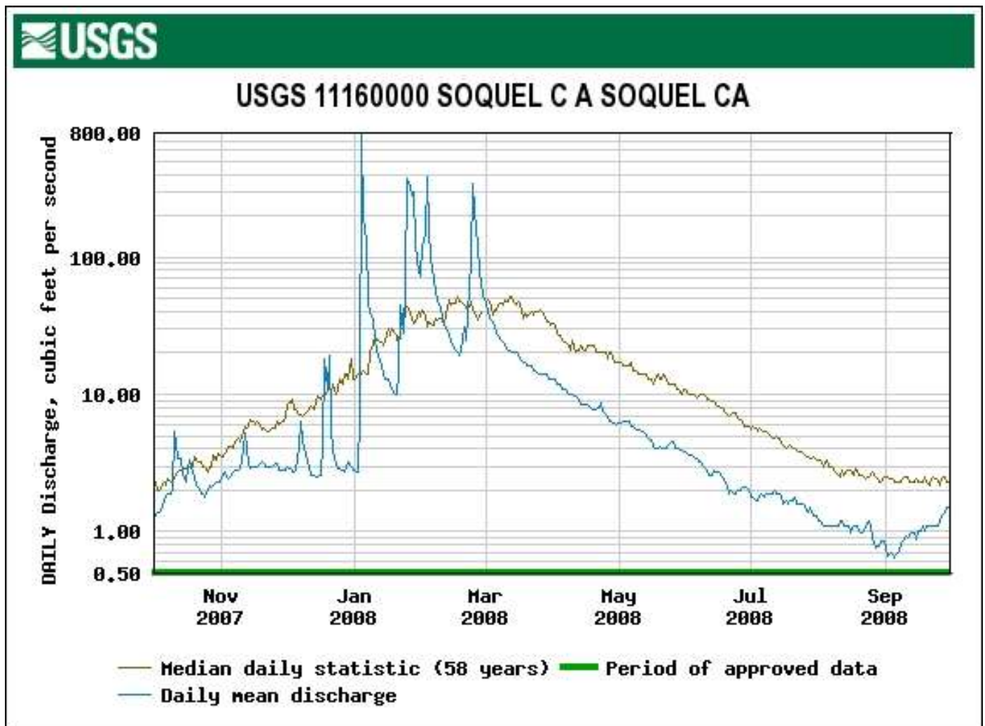
Figure 35. The 2008 Daily Mean and Median Flow at the USGS Gage on Soquel Creek at Soquel.
