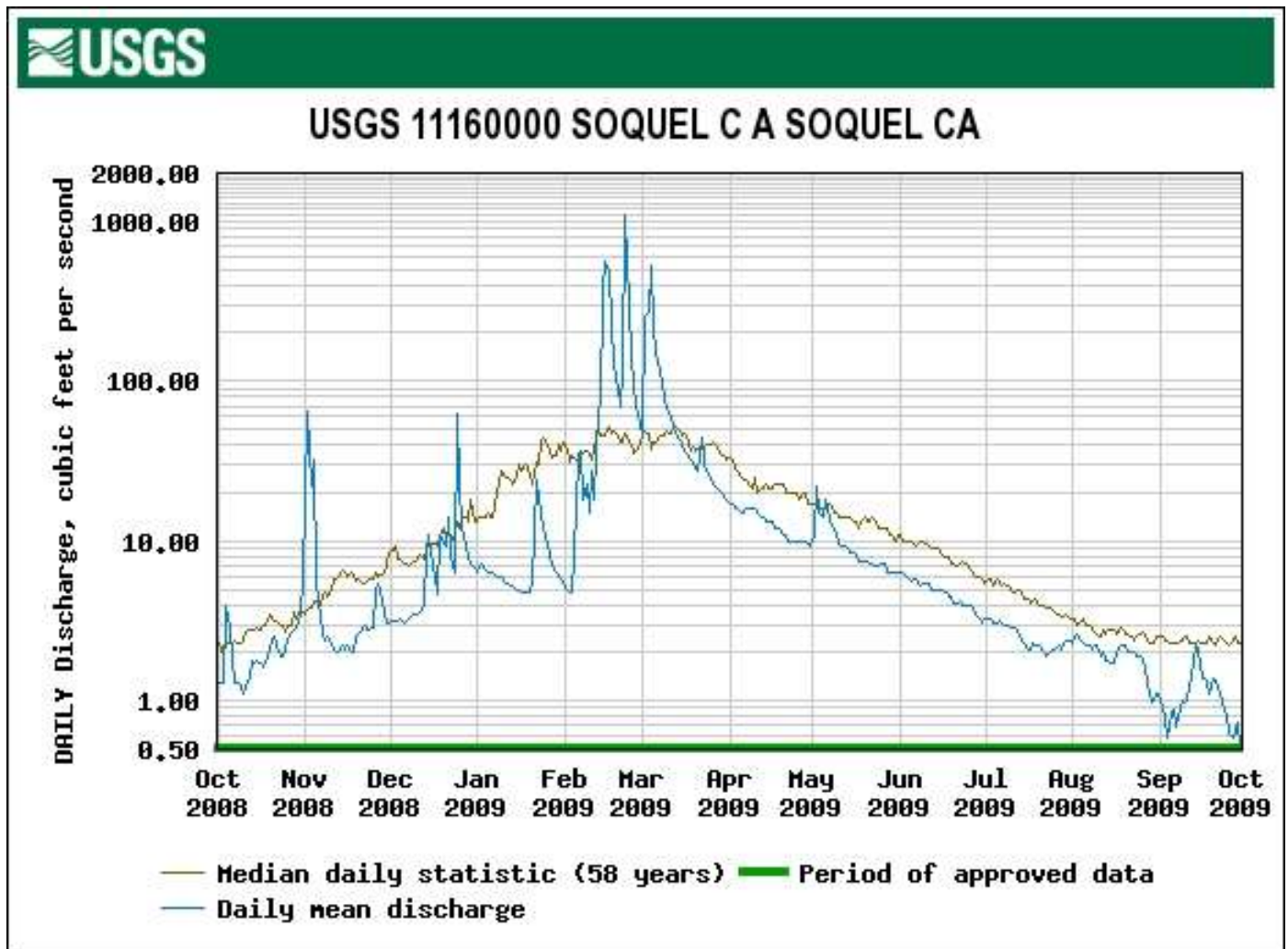
Figure 36. The 2009 Daily Mean and Median Flow at the USGS Gage on Soquel Creek at Soquel.
