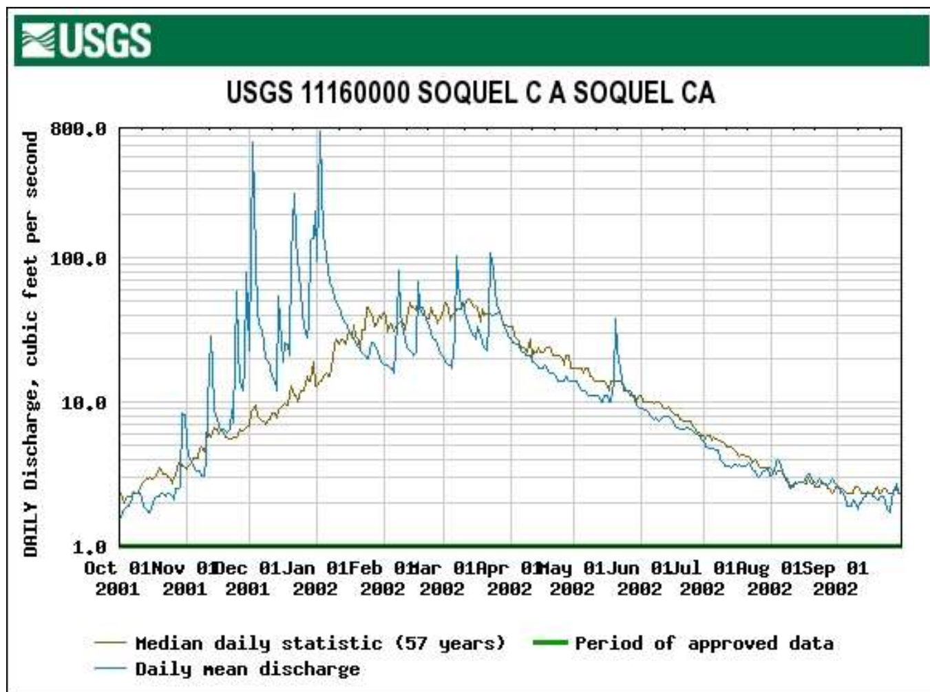
Figure 29. The 2002 Daily Mean and Peak Flood Flow at the USGS Gage on Soquel Creek at Soquel.
