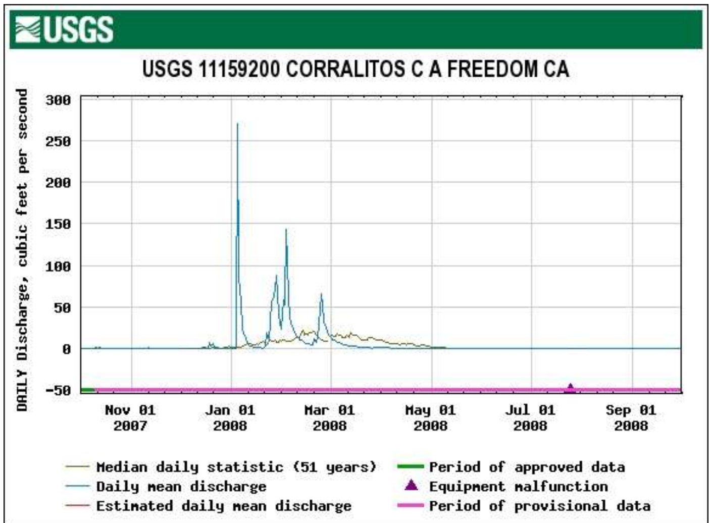
Figure 47. The 2008 Daily Mean and Median Flow at the USGS Gage on Corralitos Creek at Freedom. (USGS website would not provide a logarithmic scale of discharge).
