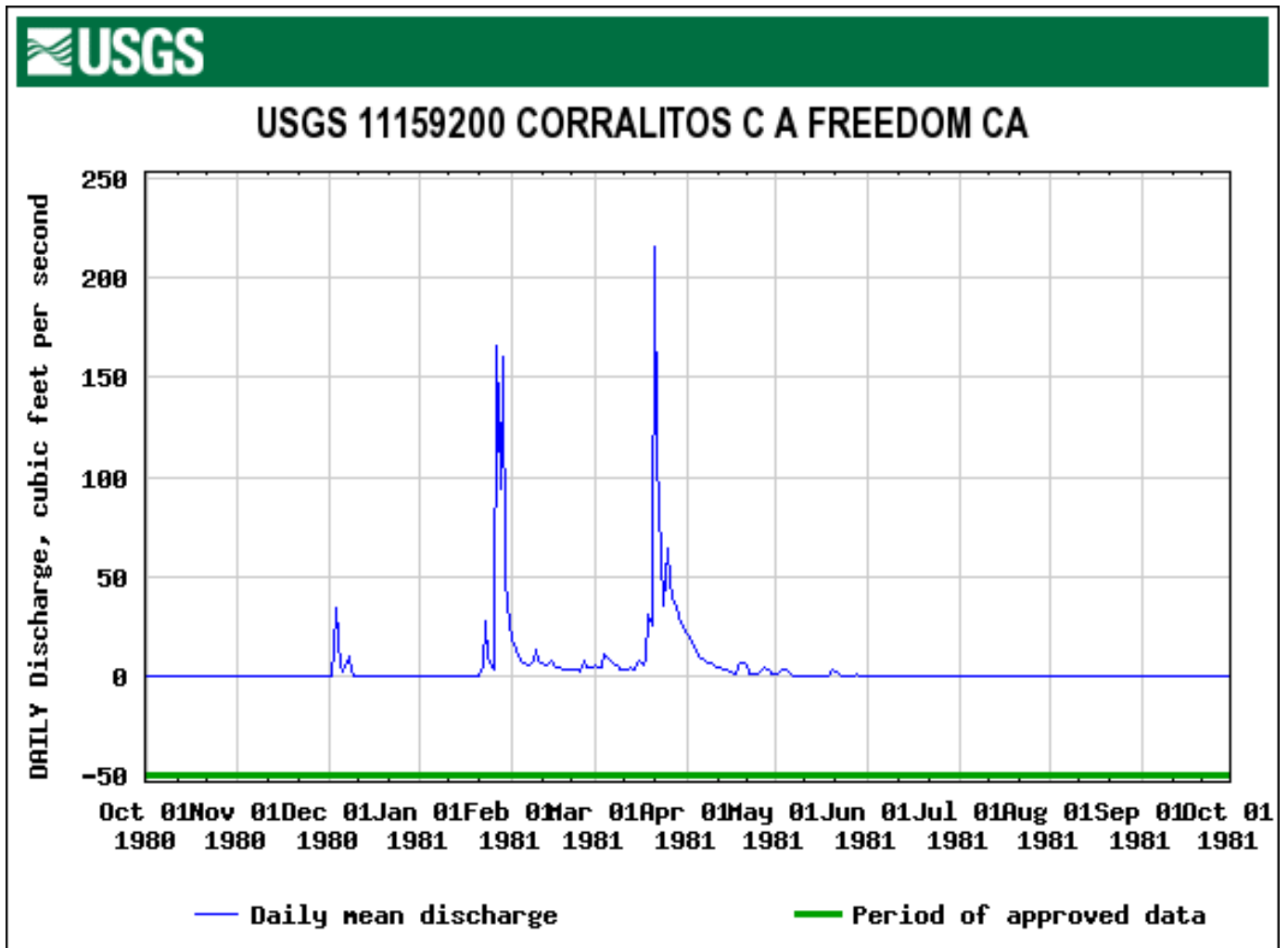
Figure 42. The 1981 Daily Mean Flow at the USGS Gage on Corralitos Creek at Freedom. (USGS website would not provide logarithmic scale of discharge.)
