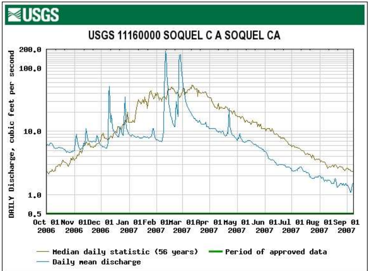
Figure 27. The 2007 Daily Mean and Median Flow at the USGS Gage on Soquel Creek at Soquel.
