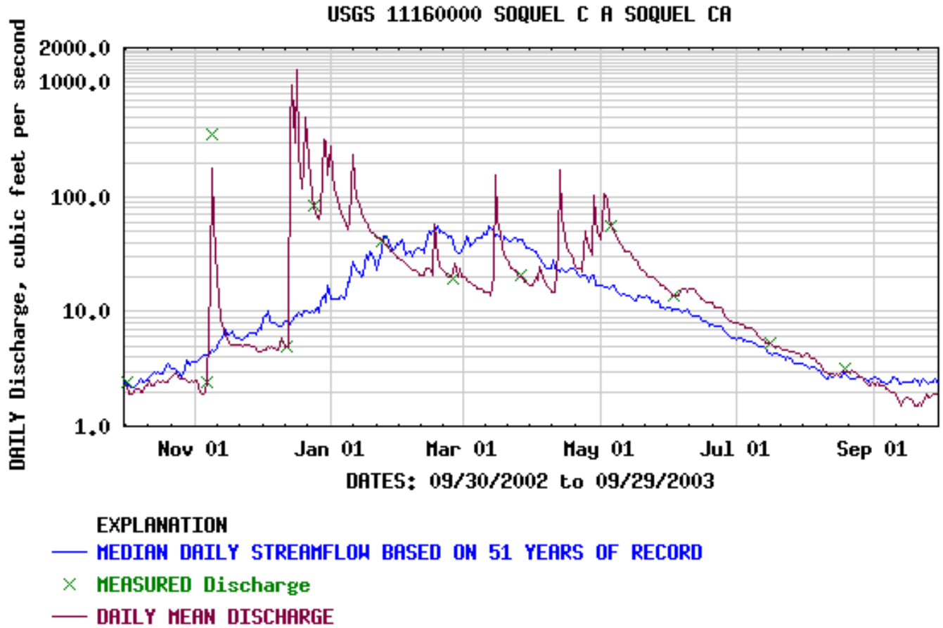
Figure 23. The 2003 Daily Mean and Median Flow at the USGS Gage on Soquel Creek at Soquel.
