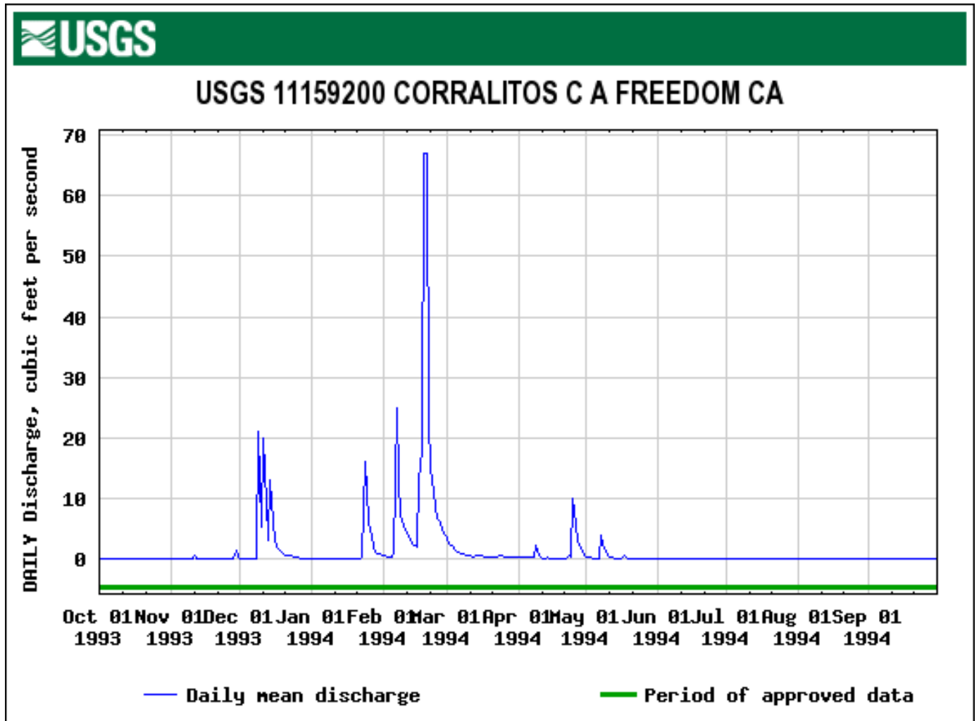
Figure 29. The 1994 Daily Mean Flow at the USGS Gage on Corralitos Creek at Freedom. (USGS website would not provide logarithmic scale of discharge.)
