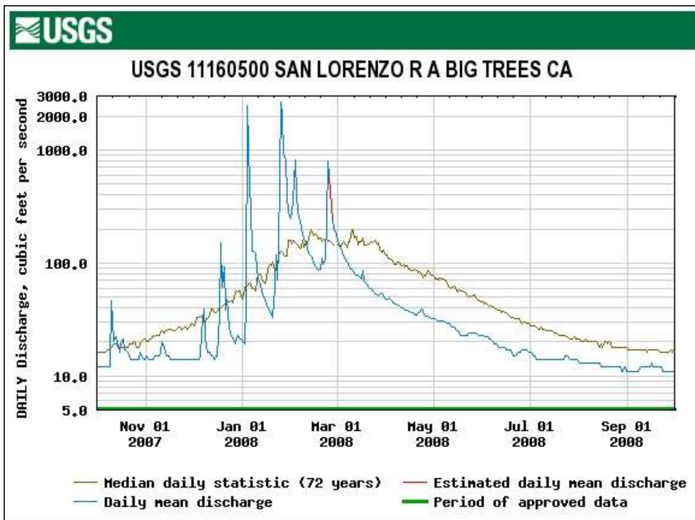
Figure 34. The 2008 Daily Average Discharge and Median Daily Flow of Record for the USGS Gage On the San Lorenzo River at Big Trees.
