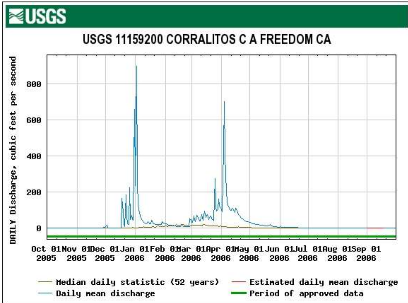
Figure 31. The 2006 Daily Mean Flow at the USGS Gage on Corralitos Creek at Freedom with Median Flow Statistics.
