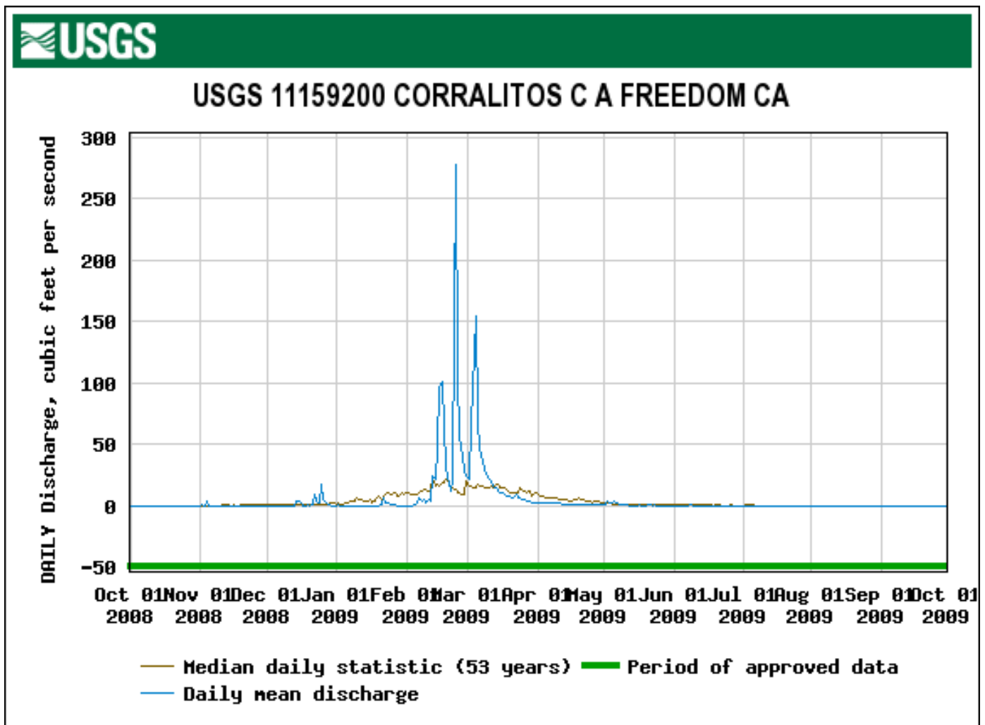
Figure 37. The 2009 Daily Mean and Median Flow at the USGS Gage on Corralitos Creek at Freedom. (USGS website would not provide a logarithmic scale of discharge).
