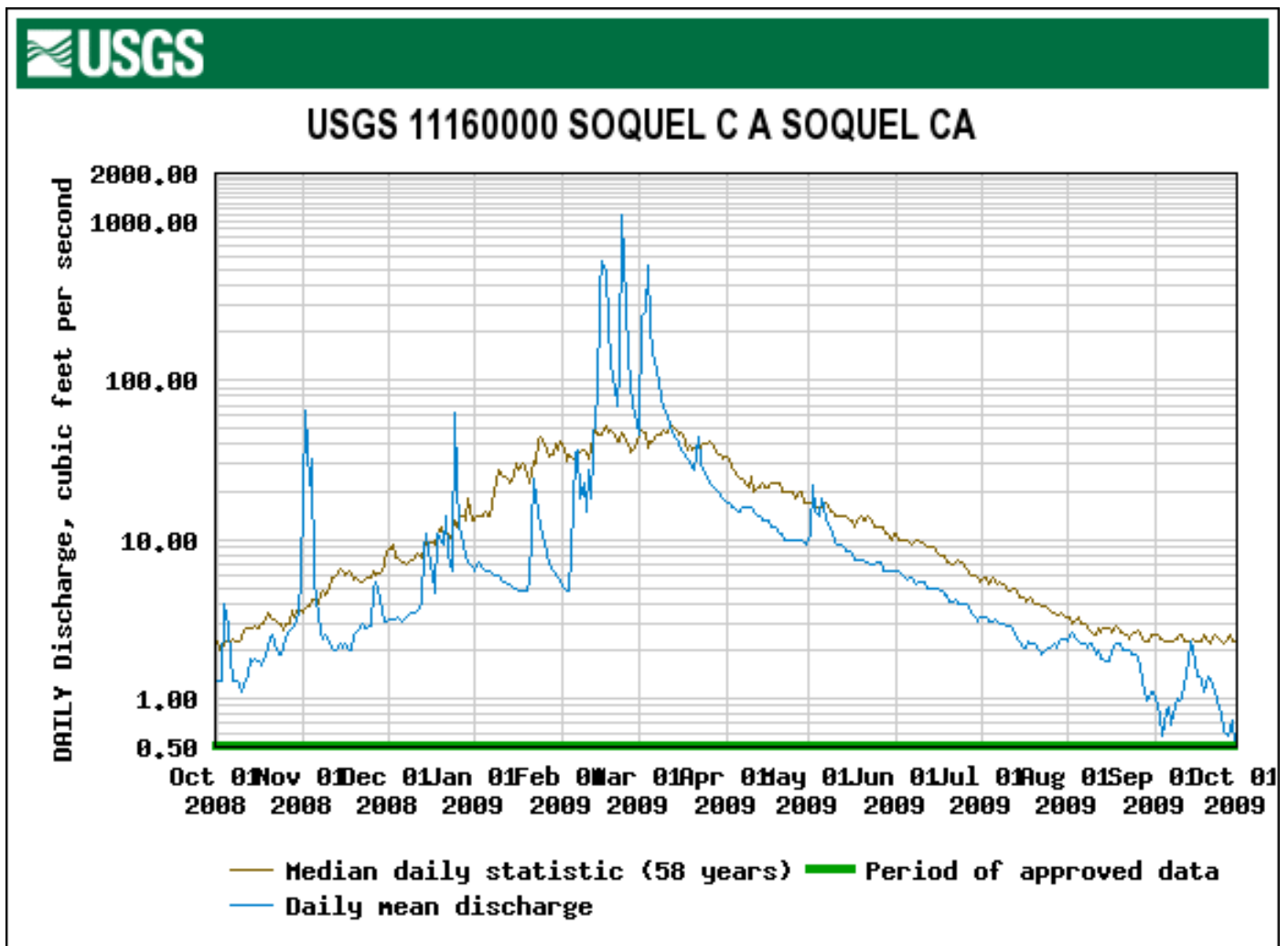
Figure 35. The 2009 Daily Mean and Median Flow at the USGS Gage on Soquel Creek at Soquel.
