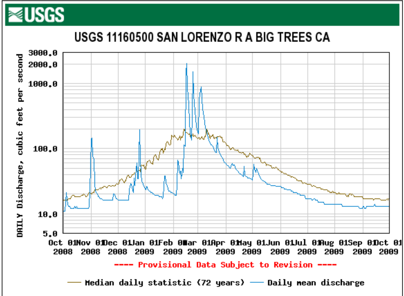
Figure 33. The 2009 Daily Average Discharge and Median Daily Flow of Record for the USGS Gage On the San Lorenzo River at Big Trees.
