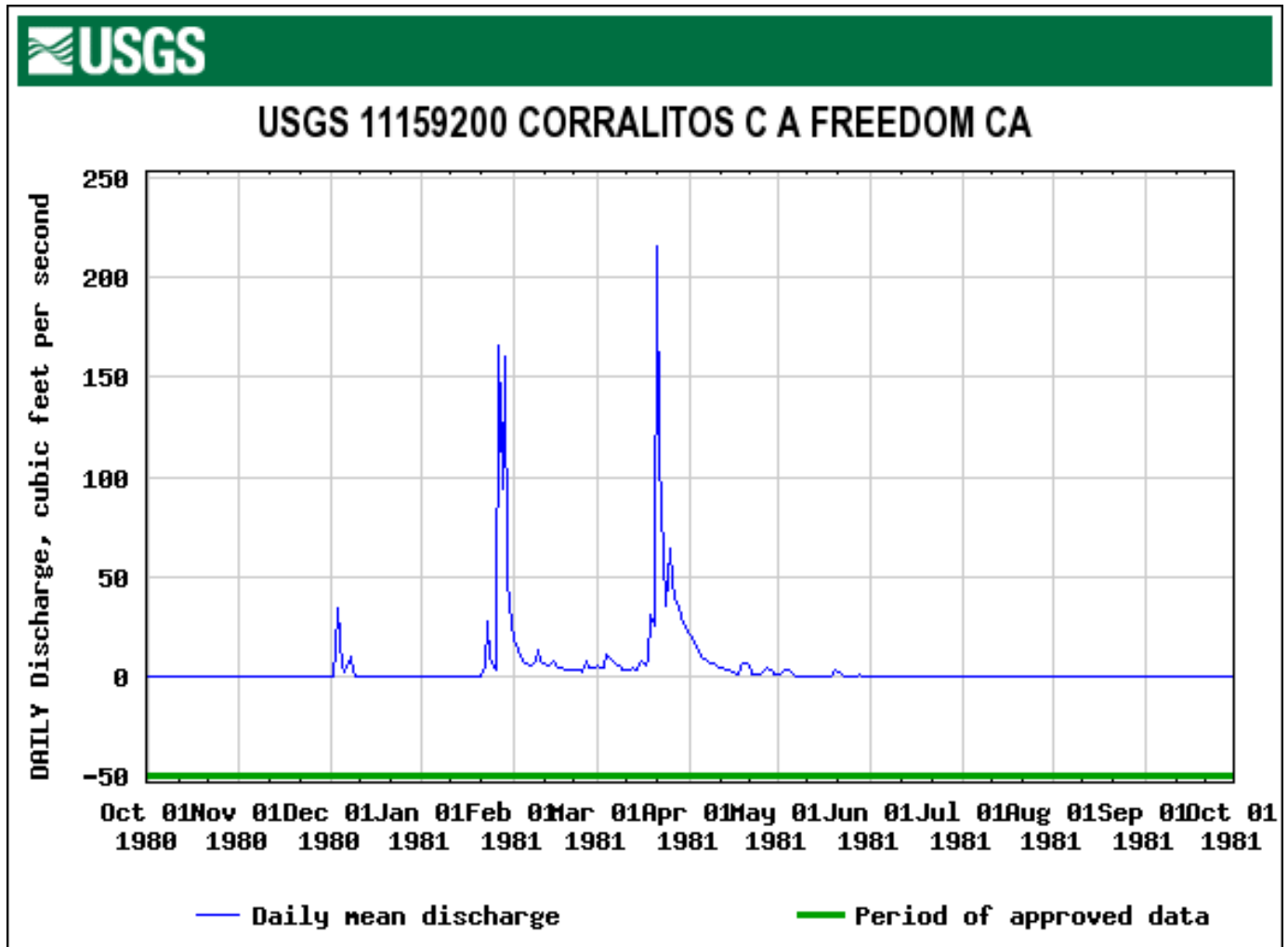
Figure 28. The 1981 Daily Mean Flow at the USGS Gage on Corralitos Creek at Freedom. (USGS website would not provide logarithmic scale of discharge.)
