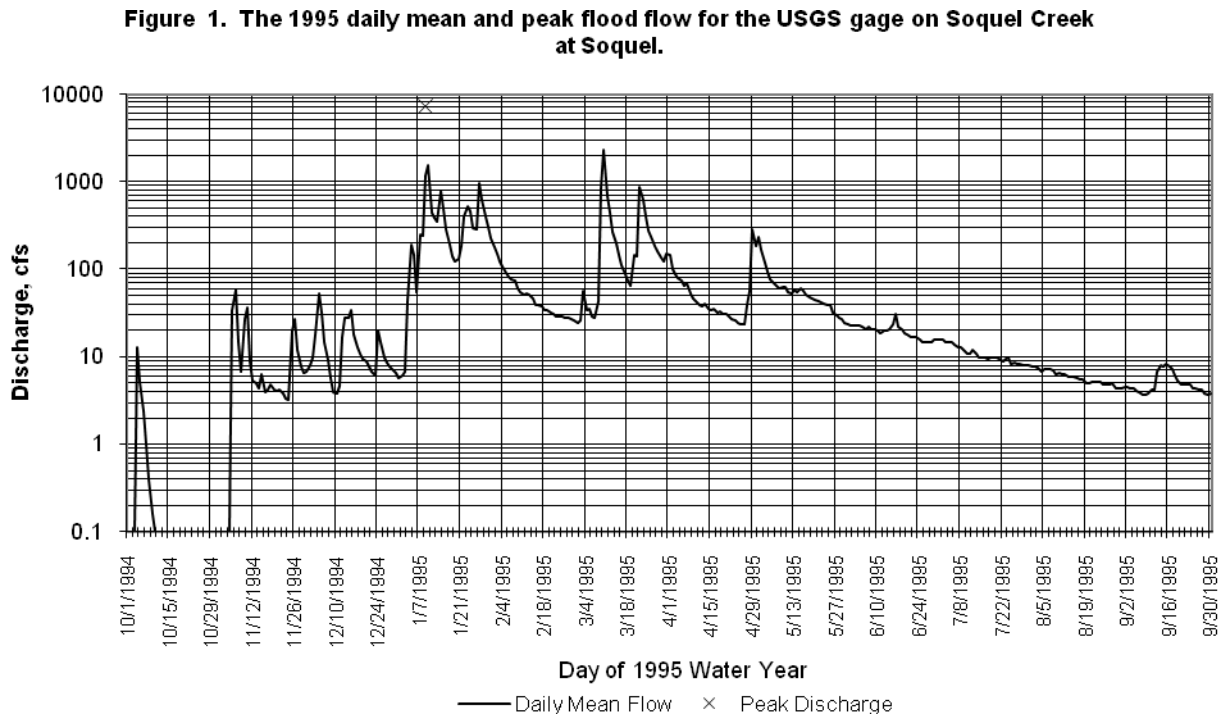
Figure 15. The 1995 Daily Mean and Peak Flood Flow at the USGS Gage on Soquel Creek at Soquel.
