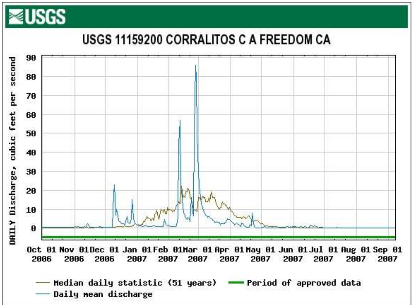
Figure 32. The 2007 Daily Mean and Median Flow at the USGS Gage on Corralitos Creek at Freedom. (USGS website would not provide a logarithmic scale of discharge).
