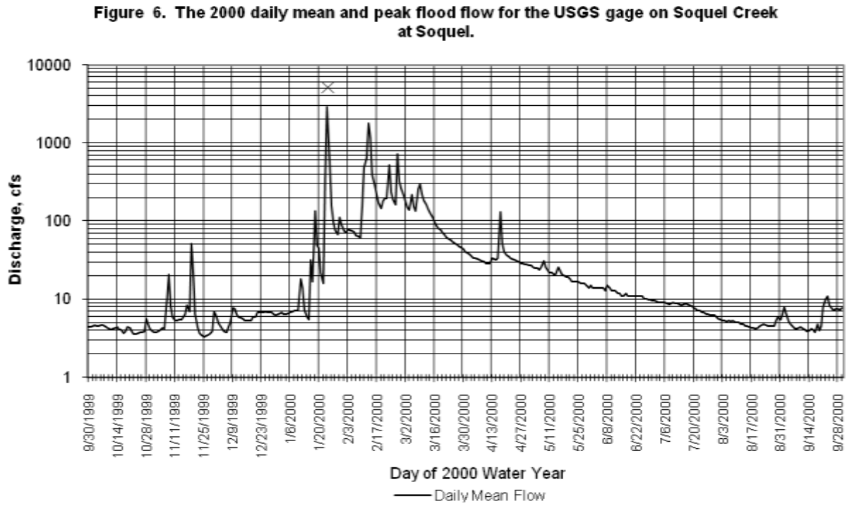
Figure 20. The 2000 Daily Mean and Peak Flood Flow at the USGS Gage on Soquel Creek at Soquel.
