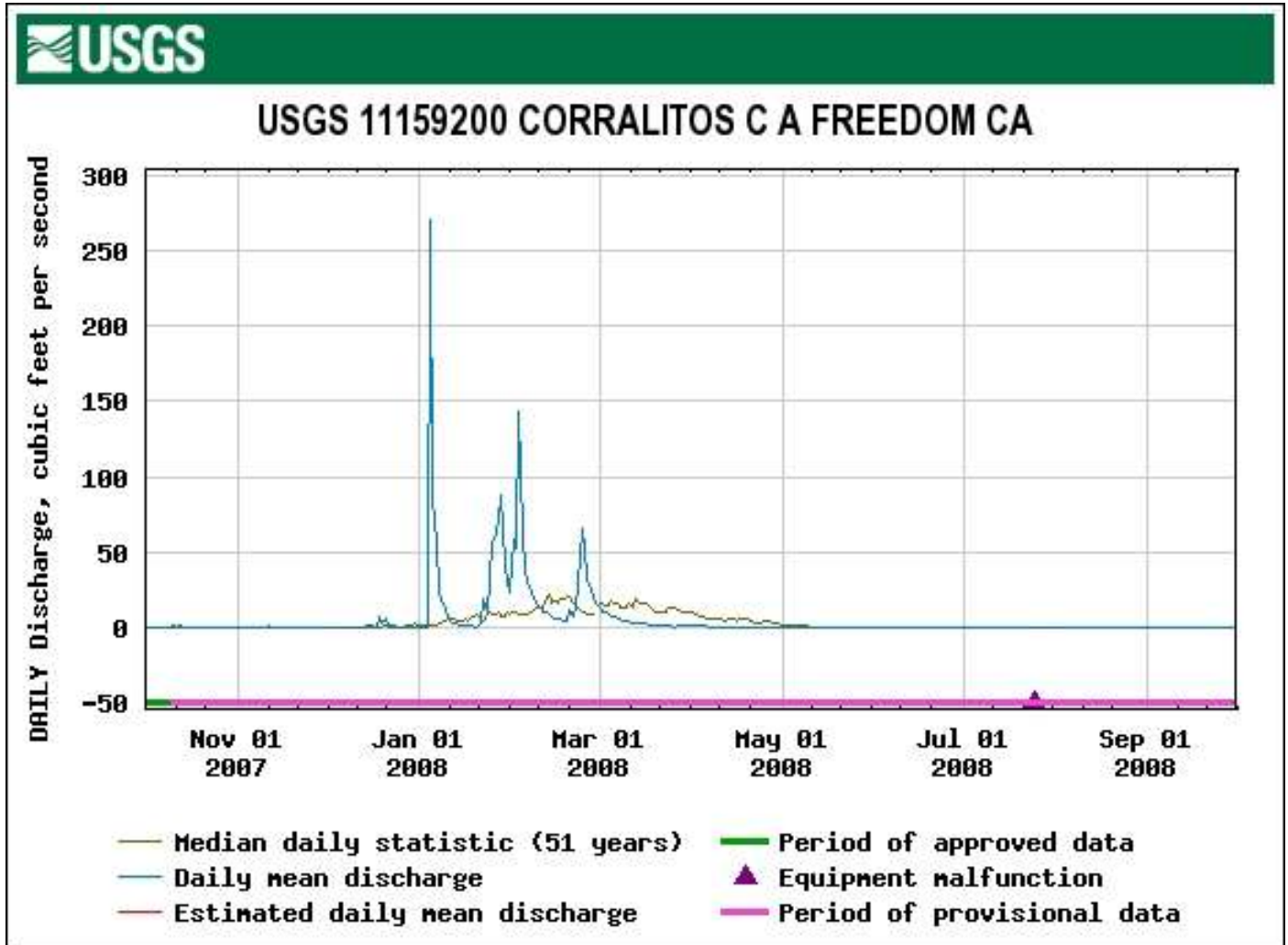
Figure 38. The 2008 Daily Mean and Median Flow at the USGS Gage on Corralitos Creek at Freedom. (USGS website would not provide a logarithmic scale of discharge).
