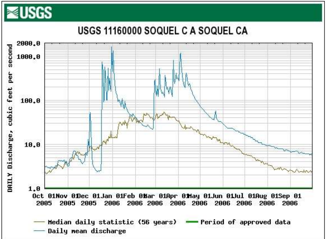
Figure 26. The 2006 Daily Mean and Median Flow at the USGS Gage on Soquel Creek at Soquel.
