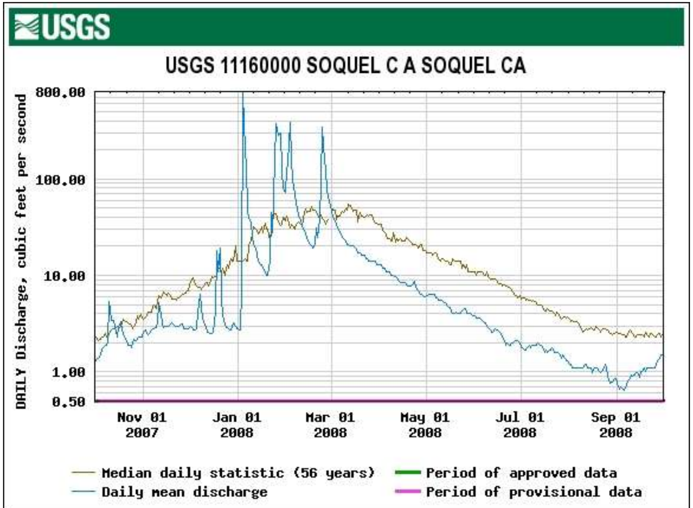
Figure 36. The 2008 Daily Mean and Median Flow at the USGS Gage on Soquel Creek at Soquel.
