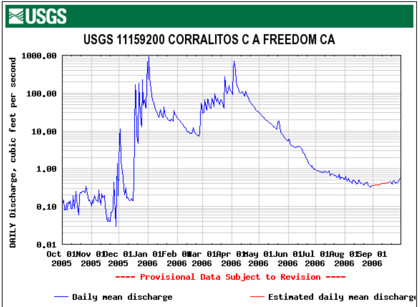
Figure 30. The 2006 Daily Mean Flow at the USGS Gage on Corralitos Creek at Freedom.
