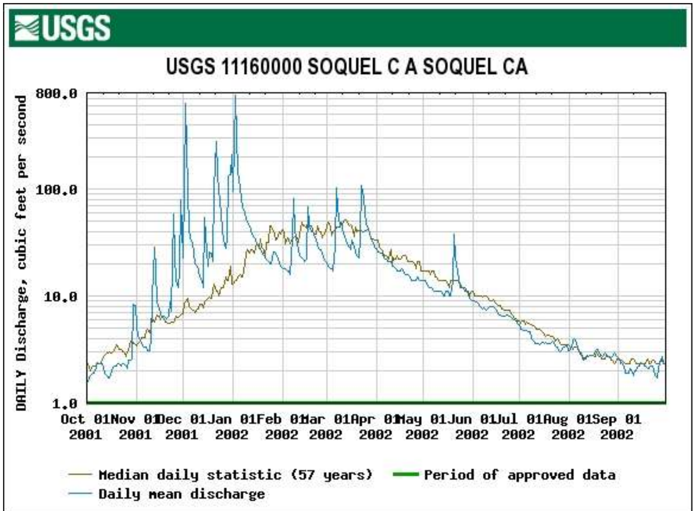
Figure 22. The 2002 Daily Mean and Peak Flood Flow at the USGS Gage on Soquel Creek at Soquel.
